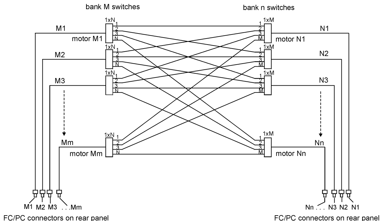
Figure 2: General Schematic of an SG MxN Switch
