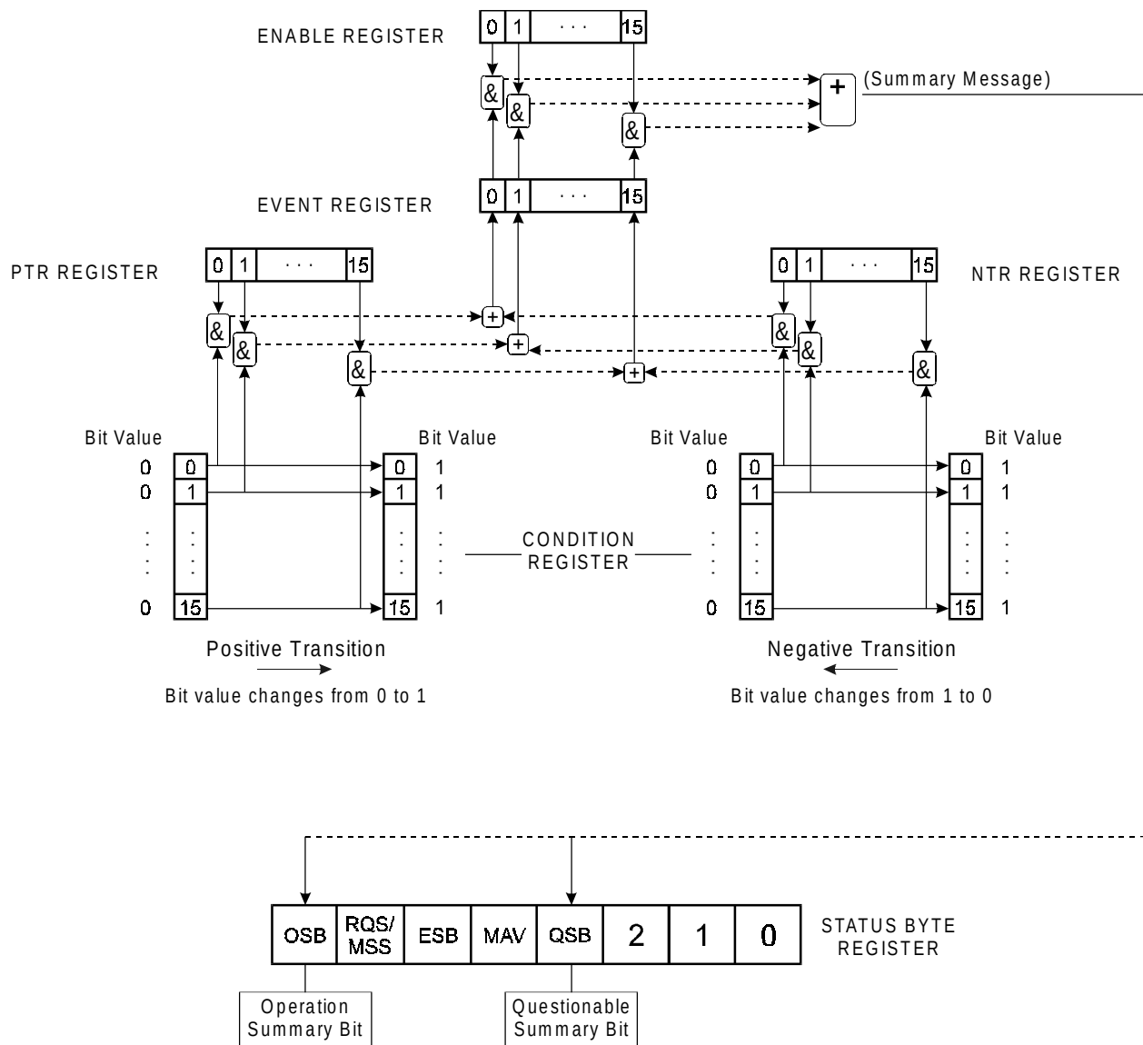
Figure 8: Data Structures
