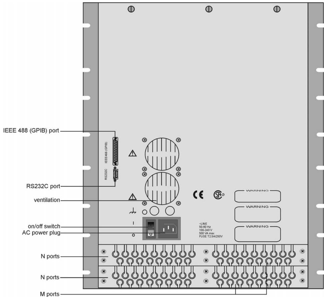
Figure 7: Back of Switch (14U height shown)
