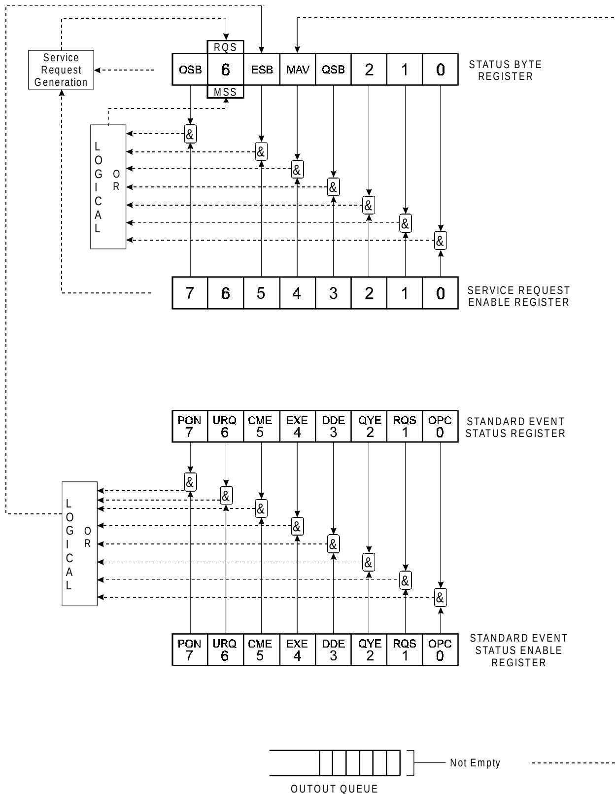
Figure 9: Registers
